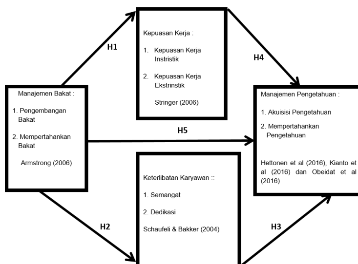
Gambar 1: Conceptual Framework
